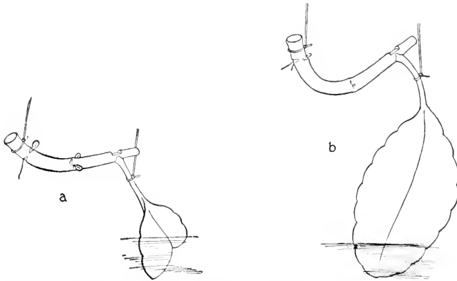
FIG. 105.—Leaf on lower side of stem. Stem b , with whole leaf, has not yet commenced to form a shoot, while the stem with a smaller piece of leaf has commenced to form shoots. May 16 to 24, 1923.
